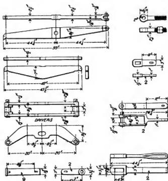
Figs. 1678-1694. Equalizers and Spring Hangers for Consolidation (2-8-0) Locomotive. American Locomotive Co.
